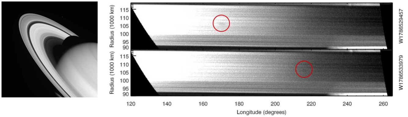
Figure 8. The last spoke seen on the lit side of the rings from the Cassini mission, from observation sequence IOSIC_207RC_COMPLRES001_SI, which was obtained on 2014 August 12, at a phase angle of 16^\circ.7 and a solar elevation angle of 22^\circ.7 . This faint dark spoke cannot be easily seen in the sample image (W1786529457) shown on the left but can be seen in the two filtered maps at the right at the locations marked by circles.
