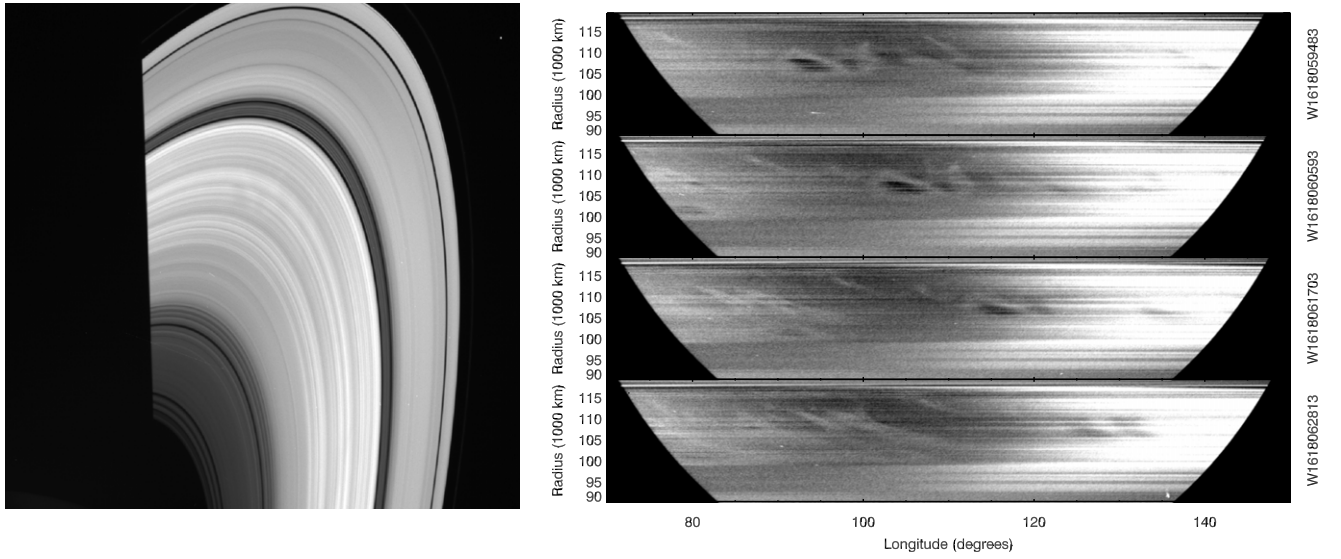
Figure 6. Mixed spokes seen on the lit side of the rings. The left image shows a representative image (W1618059483) from the observation sequence ISS_108RI_SPKMVLFLP001_PRIME, which was obtained on 2009 April 10, at a phase angle of 40^\circ and a solar elevation angle of -2^\circ.9 . Faint spokes are visible near the ansa of this image, but they are much less obvious than the spokes in Figures 2 and 3. The right image shows a series of maps derived from this sequence where the average brightness at each radius has been subtracted off to better show the signals from the spokes. These maps reveal that several spokes have dark interiors surrounded by bright edges.
