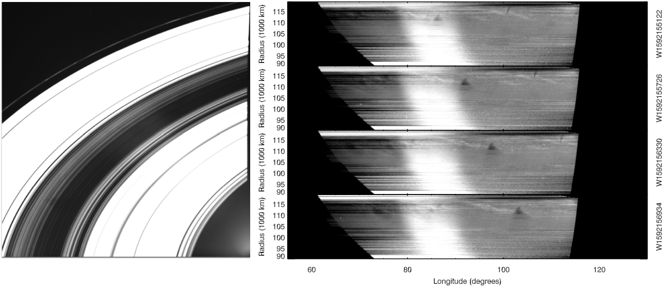
Figure 7. Mixed spokes seen on the unlit side of the rings. The left image shows a representative image (W1592156934) from the observation sequence ISS_072RI_SPKHRLPDF001_PRIME, which was obtained on 2008 June 14, at a phase angle of 32^\circ and a solar elevation angle of -6^\circ.5 . A faint dark spoke is visible at the lower left of this image, but the signals from the spokes are again relatively subtle. The right image shows a series of maps derived from images in this sequence where the average brightness at each radius has been subtracted off to better show the signals from the spokes. These maps show a dark triangular patch associated with a thin bright structure extending over 10^\circ in longitude.
