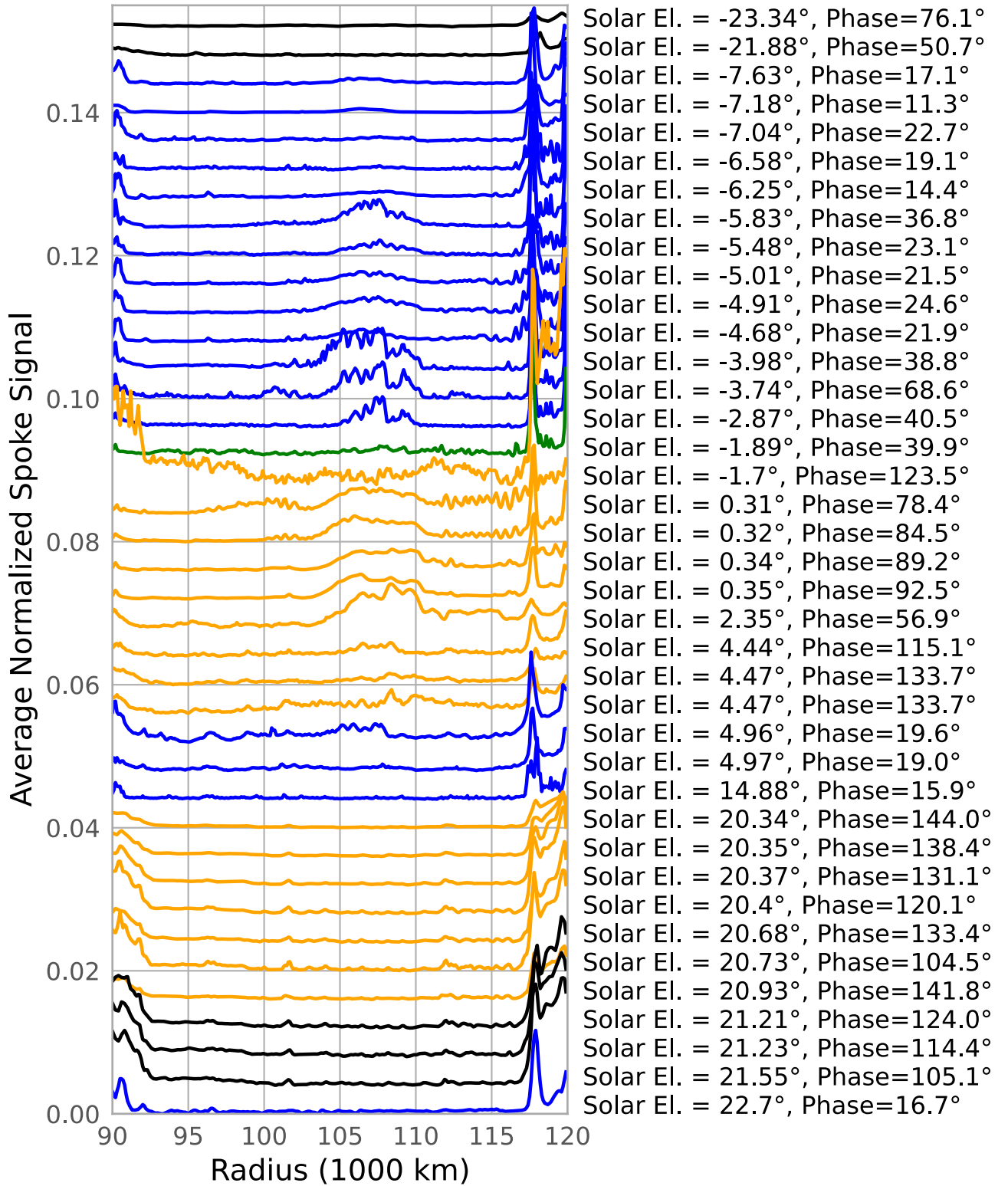
Figure 11. The averaged normalized spoke signal ( \bar{n} ) profiles for lit-side observations containing at least four images targeted at the same region of the rings. Curves are sorted by time/solar elevation angle and have been offset so the minimum values in these profiles are evenly spaced. These curves are also color coded based on the properties of observed spokes. Black curves are observations where no spoke was visible, while blue, orange, and green curves are observations where the spokes were dark, bright, or mixed, respectively. Note the clear increase in the signal between 103,000 and 112,000 km for solar elevation angles within a few degrees of zero.
