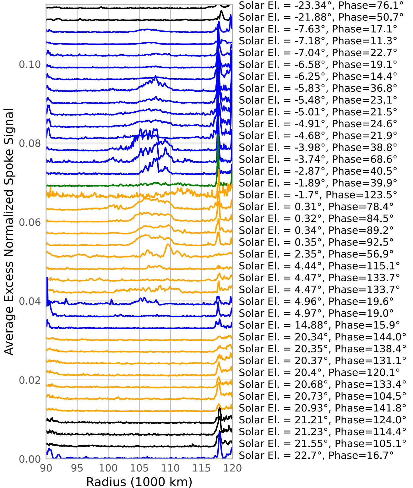
Figure 12. The average excess normalized spoke signal ( \bar{n}' ) profiles for lit-side observations containing at least four images targeted at the same region of the rings. Curves are sorted by time/solar elevation angle and are again color coded based on the properties of observed spokes. Black curves are observations where no spoke was visible, while blue, orange, and green curves are observations where the spokes were dark, bright, or mixed. Compared to Figure 11, these profiles show less structure outside of the region containing the spokes.
