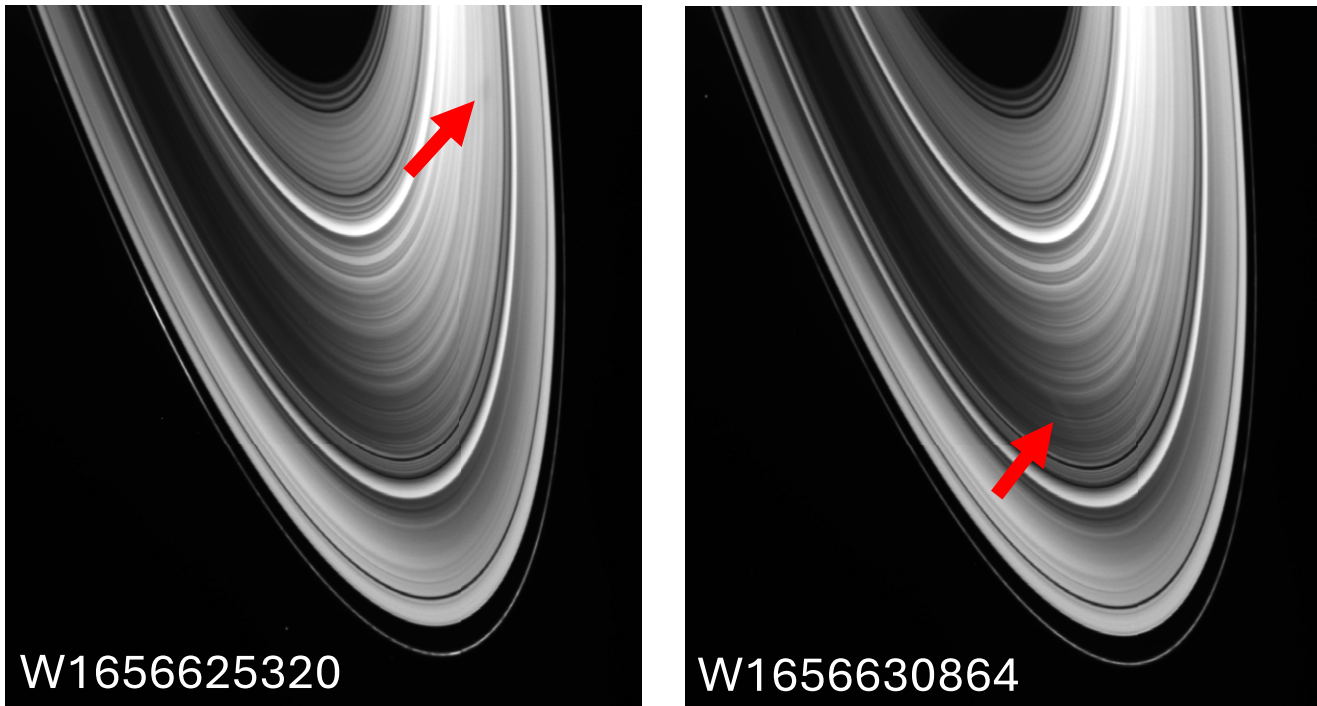
Figure 5. Representative images from the observation of the unlit side of the rings (ISS_134RI_SPKMVDHP001_PRIME) that produced the maps shown in Figure 4. Both images have arrows indicating the location of the spoke marked by the circles in Figure 4. Note that the spoke is less obvious in these images than in the maps because no filtering has been used to isolate the spoke signals. Still, the spoke does appear as a subtle dark feature against the relatively bright part of the rings in the left image and as a bright feature against the darker part of the rings in the right image.
