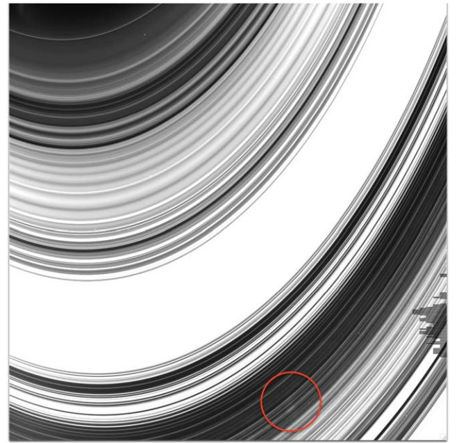
Figure 9. The last spoke seen on the unlit side of the rings from the Cassini mission, from an image (W1870770784) in observation sequence ISS_269RI_HIPHASEFB001_PIE, which was obtained on 2017 April 13, at a phase angle of 175^\circ and a solar elevation angle of 26^\circ.7 . The spoke is the bright feature marked by the circle in this particular image.
