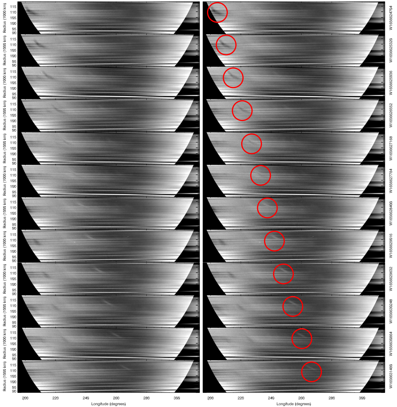
Figure 4. Example of a variable spoke from an observation of the unlit side of the rings (ISS_134RI_SPKMVDFHP001_PRIME), which was obtained on 2010 June 30, at a phase angle of 110^\circ and a solar elevation angle of 4^\circ 9' . The two columns show a series of maps (filtered so that the average brightness at each radius has been removed) where a spoke can be observed moving from left to right (marked with circles on the right set of maps). The spoke clearly goes from being darker than the background ring at the start of the sequence to being brighter than the background ring near the end of the sequence.
