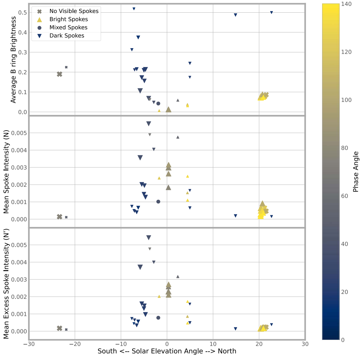
Figure 13. Timelines of average spoke intensity over the course of the Cassini mission derived from the profiles shown in Figures 11 and 12. The shapes of the data points indicate the types of spokes visible in the images, and their sizes indicate the number of images considered in each observation, while the color indicates the observed phase angle. The top panel shows the average brightness of the B ring between 102,000 and 112,000 km. Note that the brightness has a minimum at equinox and declines rapidly between solar elevation angles of -10^\circ and -5^\circ . The bottom two panels show the mean normalized spoke signal ( \bar{n} ) and mean excess normalized spoke signal ( \bar{n}' ) between 102,000 and 112,000 km above background levels, which show a clear rise and fall around equinox.
