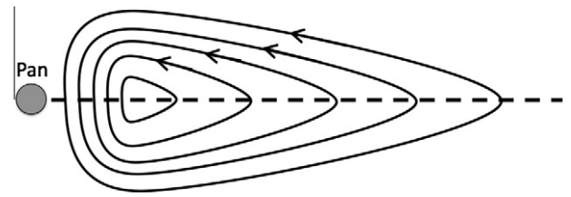
Fig. 23. Schematic representation of the asymmetric trajectories of the particles in the Pan ringlet due to the combined action of drag forces and Pan's gravity in a reference frame that co-rotates with Pan. Note radius increases upwards in this diagram, longitude increases to the left, and Pan's orbit is displayed as the dashed line. Also note that in this cartoon the radial (vertical) scale is highly exaggerated relative to the longitudinal (horizontal) scale. The particles are assumed to remain on nearly circular orbits in this cartoon, and initially have a range of longitudes along Pan's semi-major axis. On the right side of the figure, the particles are drifting outwards due to drag forces, while on the left they are undergoing horseshoe motion due to Pan's gravitational perturbations. Due to the intrinsic asymmetry of these motions, these particles are more likely to be found just in front of Pan, which is also where the clumps are located.
