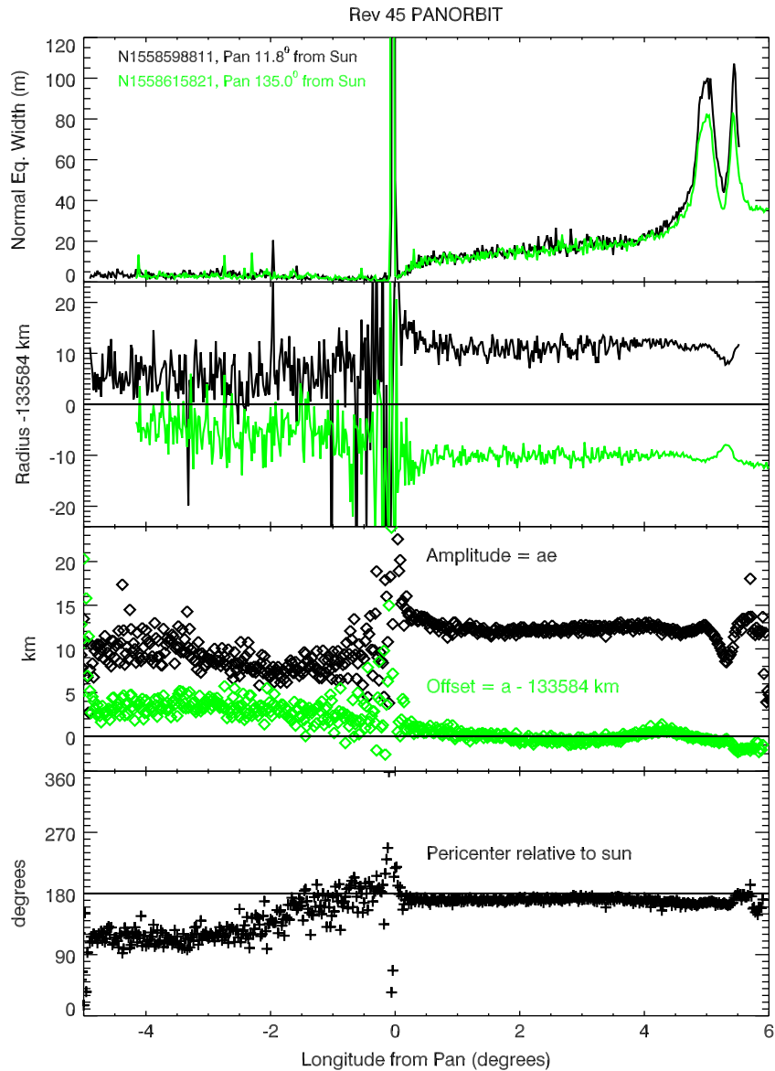
Fig. 16. Orbital elements of the Pan ringlet derived from the PANORBIT observation. The top two panels show the integrated brightness and radial position of the Pan ringlet derived from two images, one taken close to the sub-solar longitude, and the other taken near Saturn's shadow. Note that the ringlet is found displaced outward from Pan's orbit on the sunward side of the rings, and inwards on the side near Saturn's shadow. The bottom two panels show the ringlet's semi-major axis, eccentricity and pericenter longitude derived from all the useful images in this sequence. Statistical error bars are not plotted for reasons of clarity, but are consistent with the scatter in the estimates (i.e., they are around 0.5 km in a and ae and 5^\circ in the pericenter in front of Pan, and 1–2 km in a and ae and 10\text{--}20^\circ in the pericenter behind Pan). In front of Pan, the ringlet has a semi-major axis close to that of Pan, a finite eccentricity, and a pericenter anti-aligned with the Sun. Note that the eccentricity is reduced in the vicinity of the bright clumps between 5^\circ and 6^\circ . Behind Pan, where the ringlet is fainter, the semi-major axis is systematically outside the orbit of Pan and the pericenter deviates from exactly 180^\circ .
